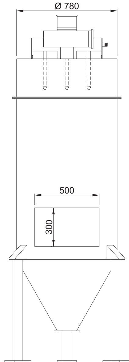
VISTA FRONTAL
